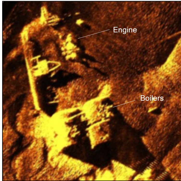
Side scan image showing boiler and engine contacts
