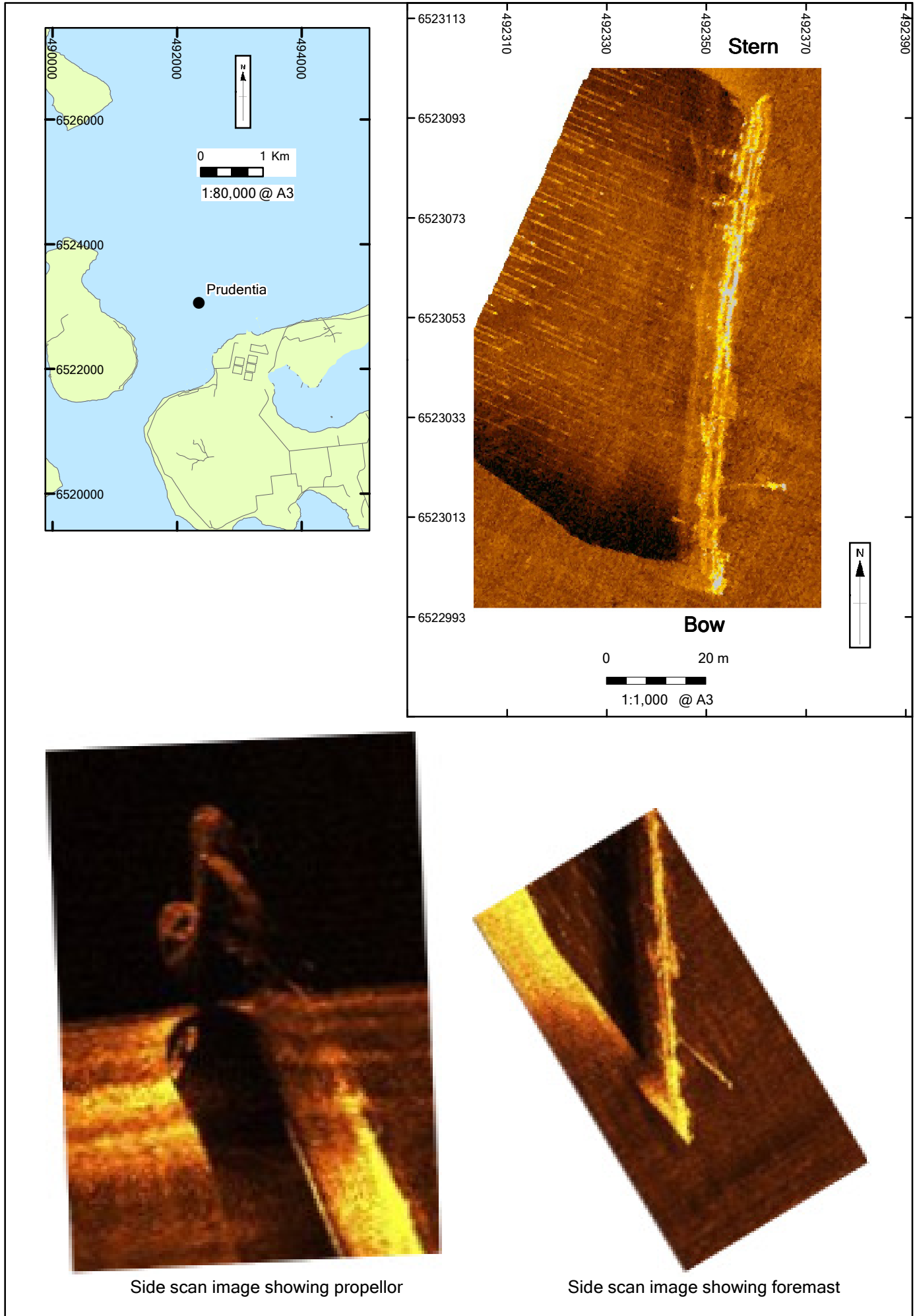
Figure 25: Side scan images from Prudentia
