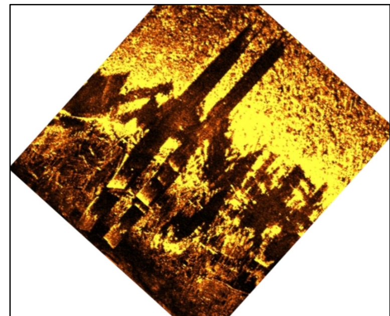
Side scan image showing boilers
