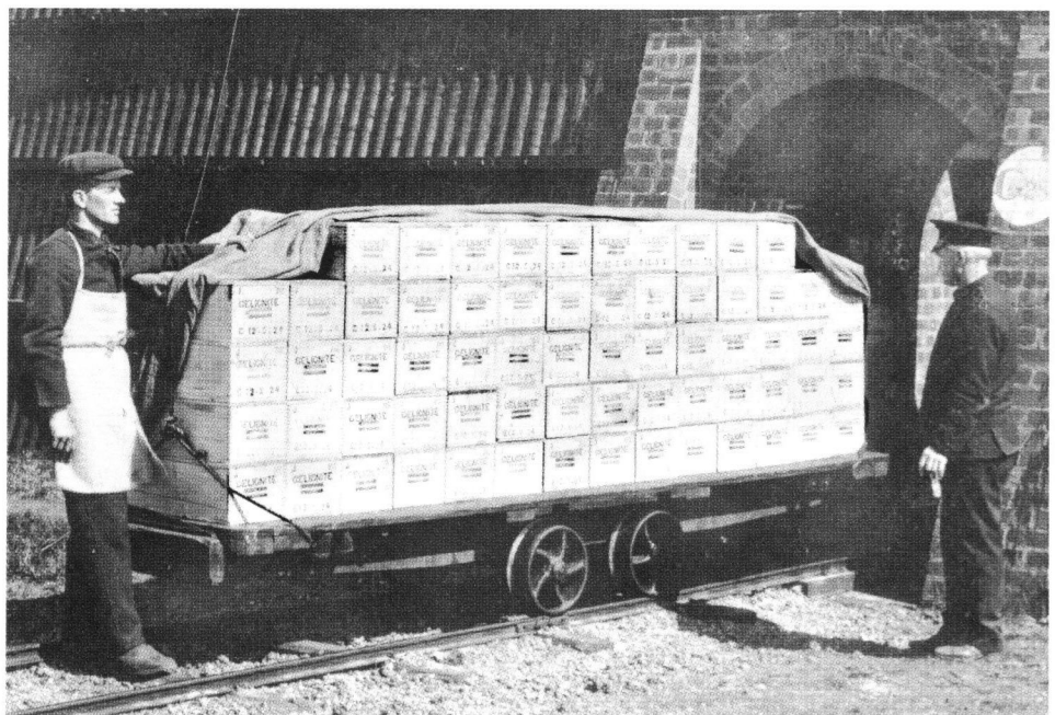
Plate 46: Blasting Department: view of bogey with finished cases of Gelignite leaving a packing house on the narrow gauge railway, and being taken for storage in a Magazine. The view also illustrates the steel-re-inforced mounds surrounding these and other types of building in the Danger Areas, circa 1925 (ICI Explosives, C65514)
