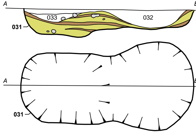
Fig. 15 - Plans and section of Roman Field Ovens 031
