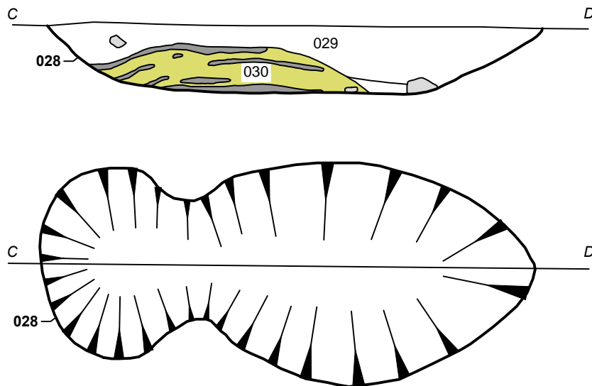
Fig. 16 - Plans and section of Roman Field Ovens 028
